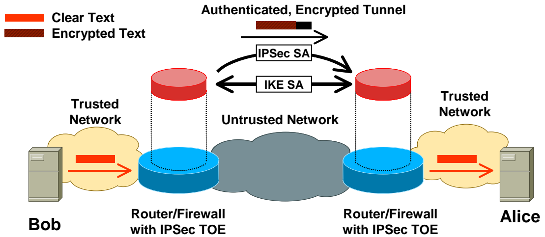
Figure 5 IPsec and IKE Operation
