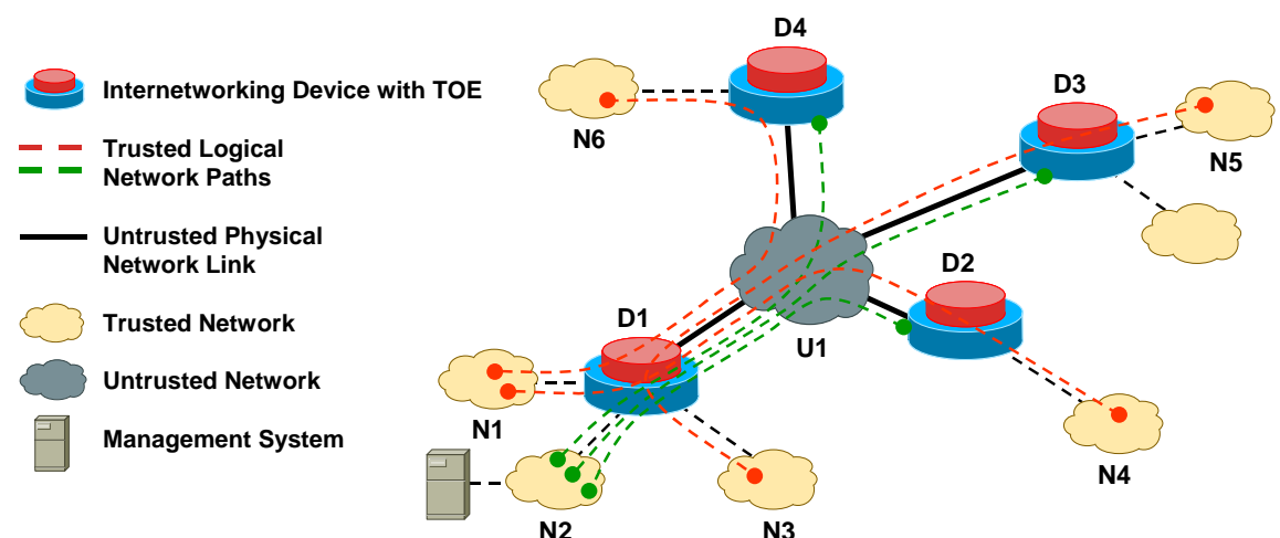
Figure 2 Organizational Security Policy Example
