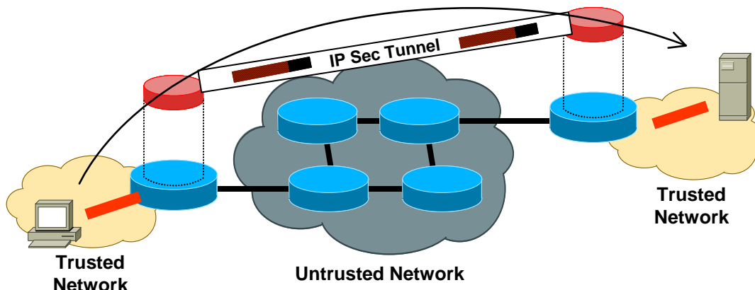
Figure 3 IPSec Tunnel Mode
