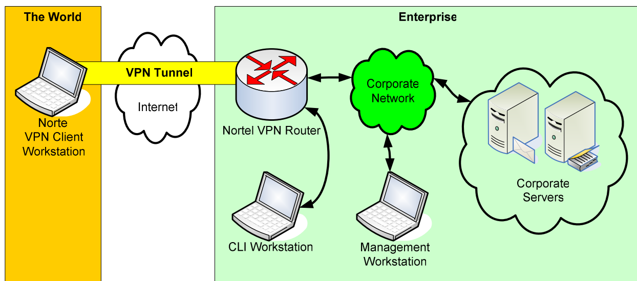
Figure 1 – VPN Client Deployment Configuration of the TOE
