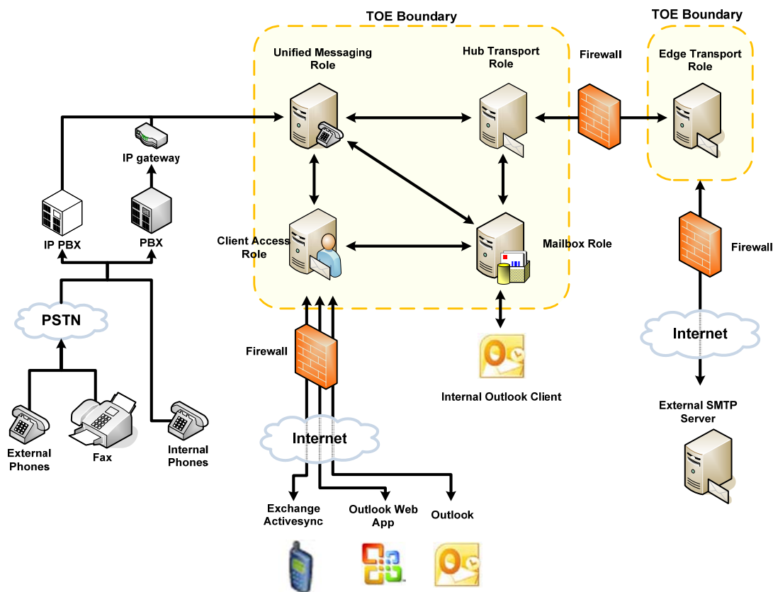
Figure 1 – Exchange 2010 architecture
