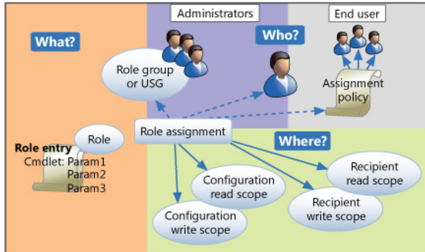
Figure 2 – RBAC Overview
